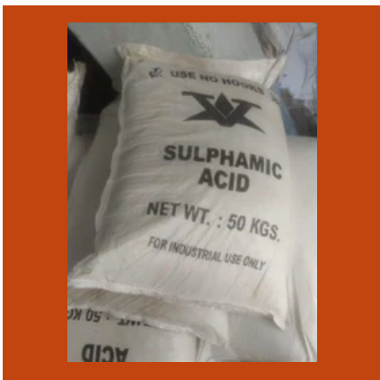
Sulphamic Acid
